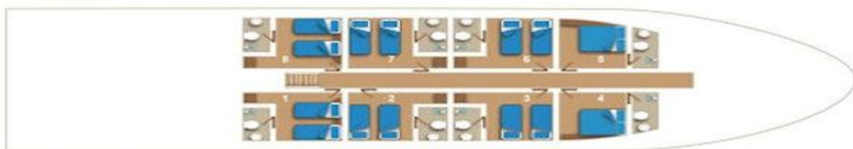
Cabin Deck (Lower Deck)
